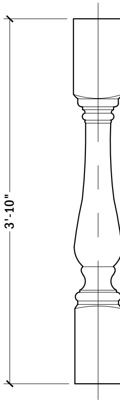
ELEVATION VIEW
