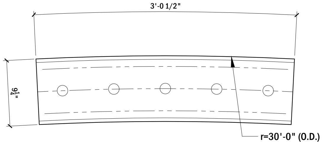
PLAN VIEW, BASE RAIL #148
