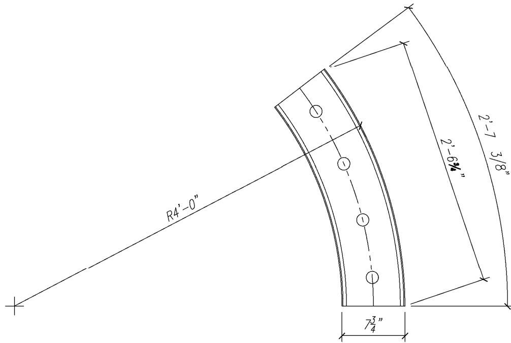
TOP VIEW
