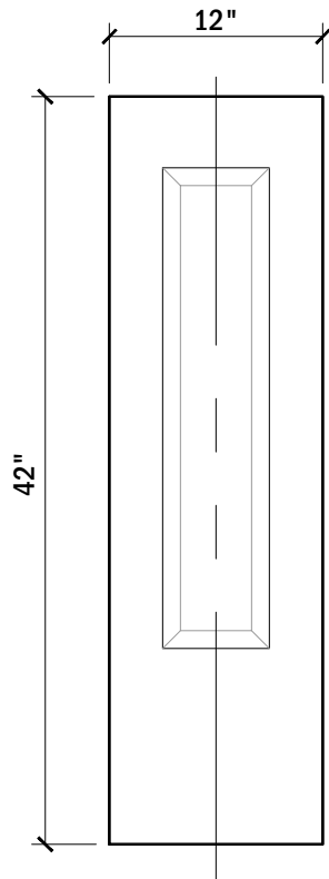
ELEVATION VIEW
