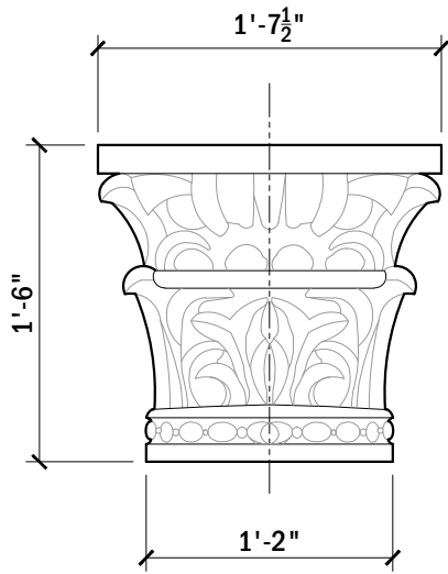
ELEVATION VIEW
