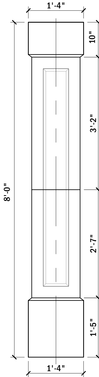
ELEVATION VIEW
