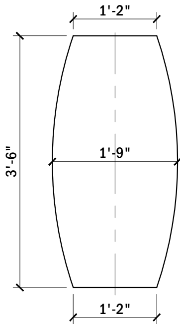
ELEVATION VIEW
