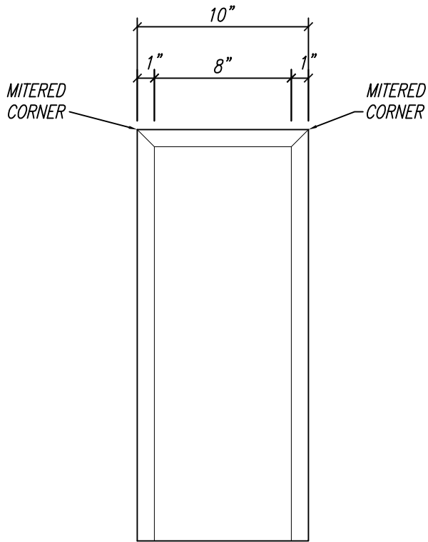
PLAN VIEW
