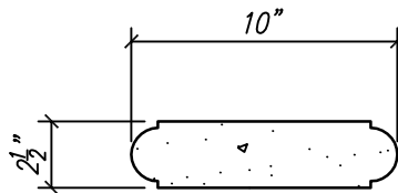
PROFILE VIEW
