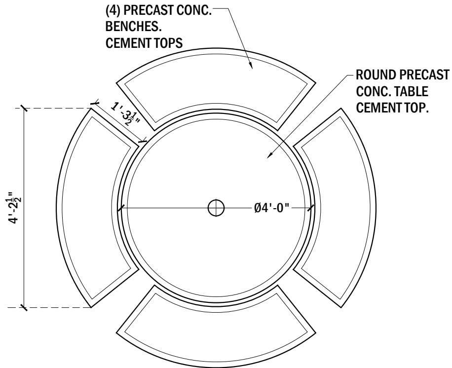
PLAN VIEW, TABLE #610
