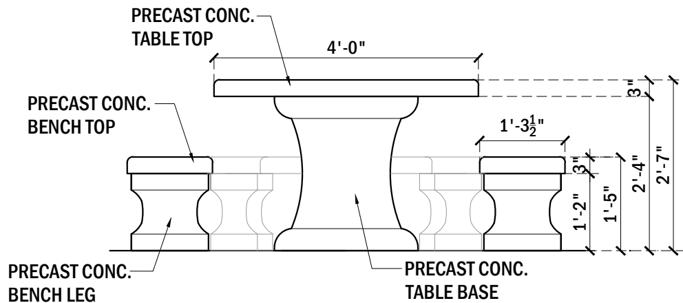
ELEVATION VIEW, TABLE #610
