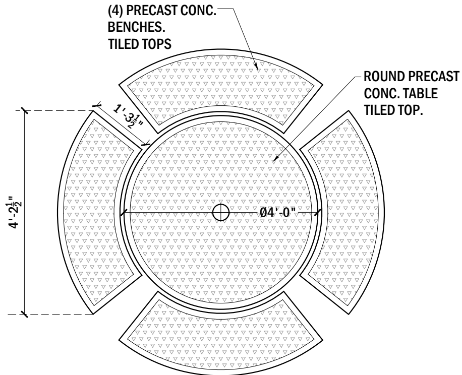
PLAN VIEW, TABLE #611
