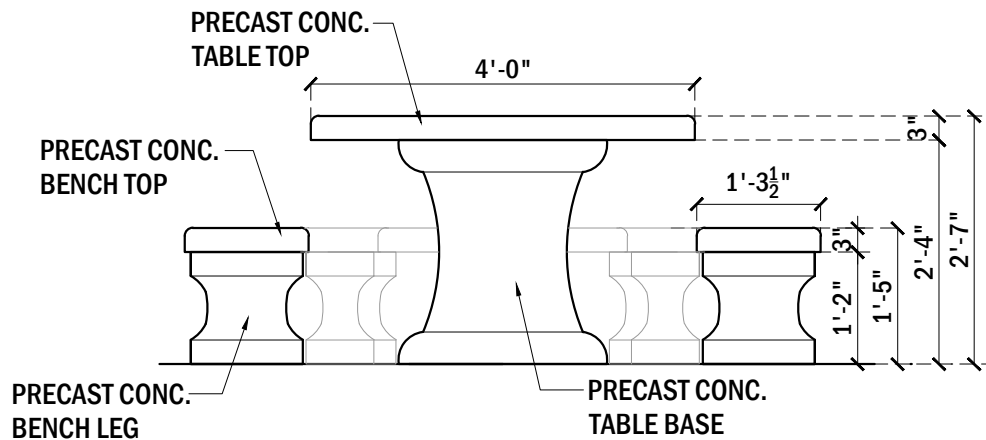
ELEVATION VIEW, TABLE #611
