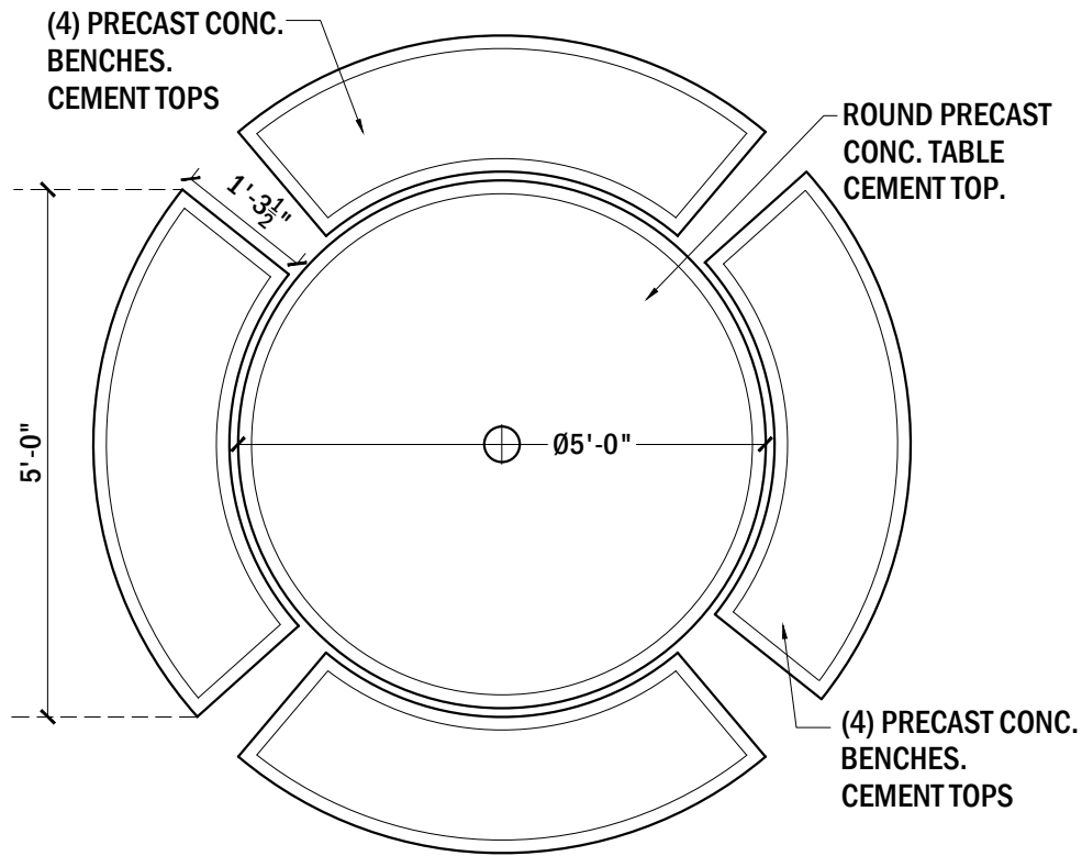
PLAN VIEW, TABLE #613
