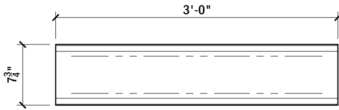
TOP VIEW, TOP RAIL #123
