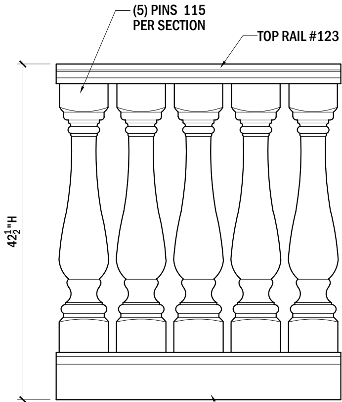
ELEVATION VIEW
