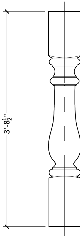
ELEVATION VIEW
