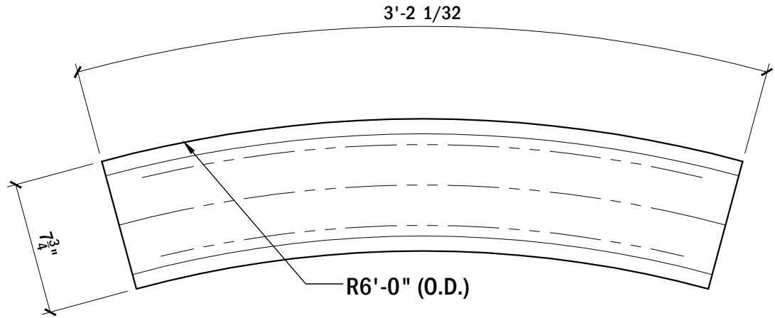
TOP VIEW, TOP RAIL #125
