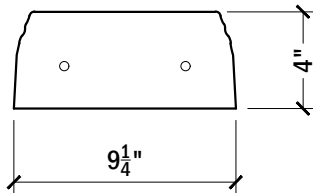
SIDE VIEW BASE RAIL #137
