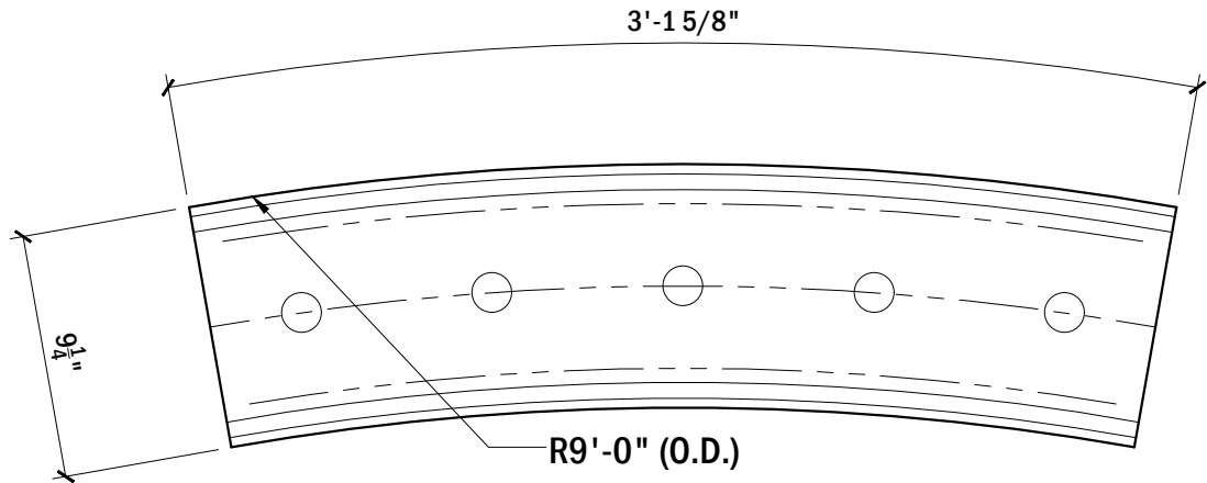
TOP VIEW, BASE RAIL #138
