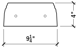
SIDE VIEW BASE RAIL #138
