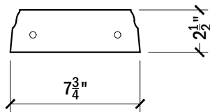
SIDE VIEW BASE RAIL #161
