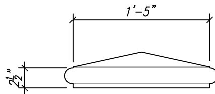
ELEVATION VIEW
